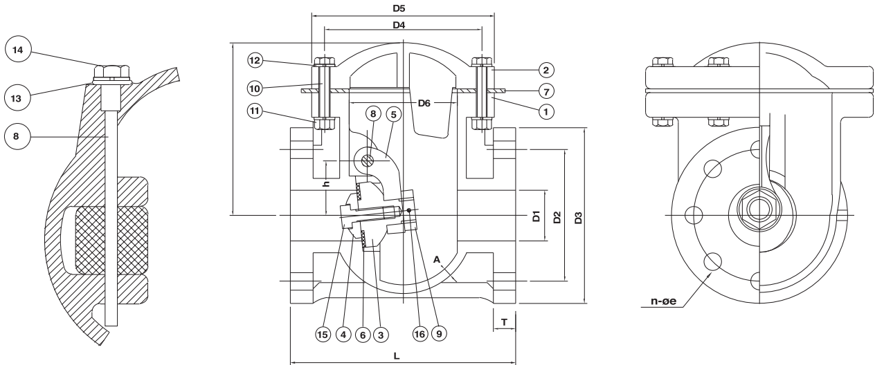
DN25~DN200
